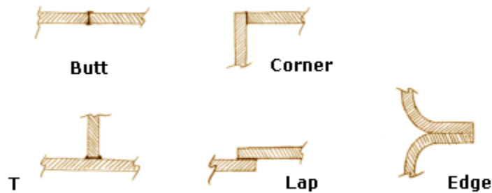
TYPES OF WELD JOINTS
